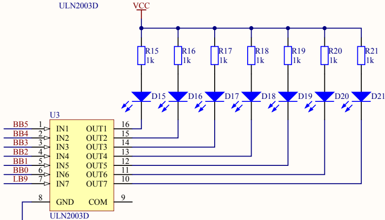
ULN2003D
