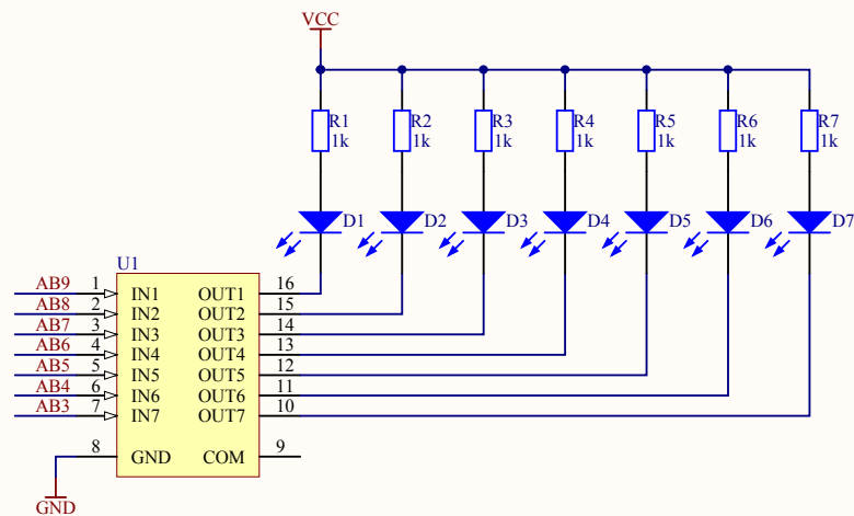
ULN2003D
