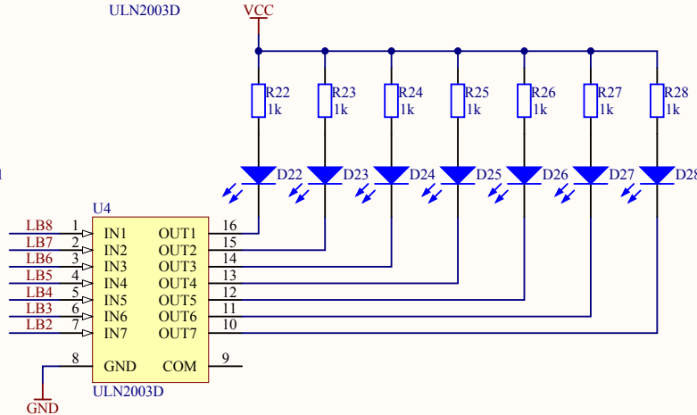
ULN2003D
